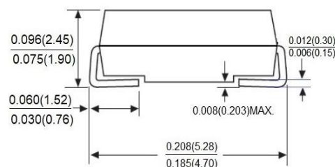
Package Outline Dimensions in Inches (Millimeters)
