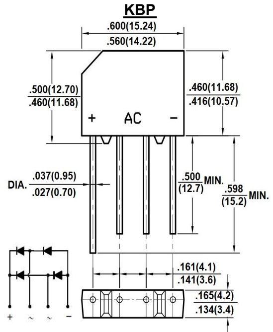
Package Outline Dimensions in Inches (Millimeters)
