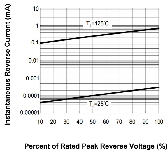
FIG. 4- TYPICAL REVERSE LEAKAGE
