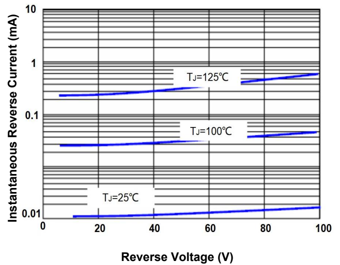
FIG. 4- TYPICAL REVERSE LEAKAGE
