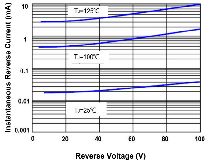
FIG. 4- TYPICAL REVERSE LEAKAGE
