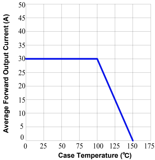
FIG. 1- DERATING CURVE OUTPUT RECTIFIED
