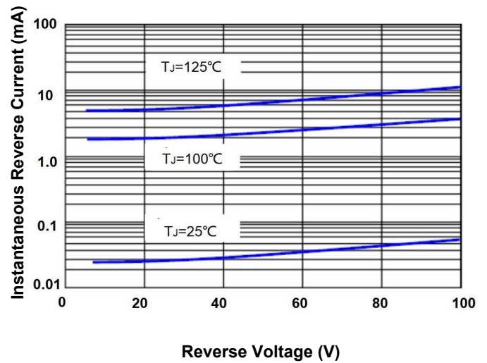
FIG. 4- TYPICAL REVERSE LEAKAGE
