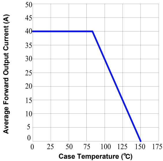
FIG. 1- DERATING CURVE OUTPUT RECTIFIED
