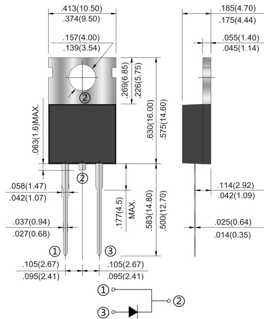
Package Outline Dimensions in Inches (Millimeters)
