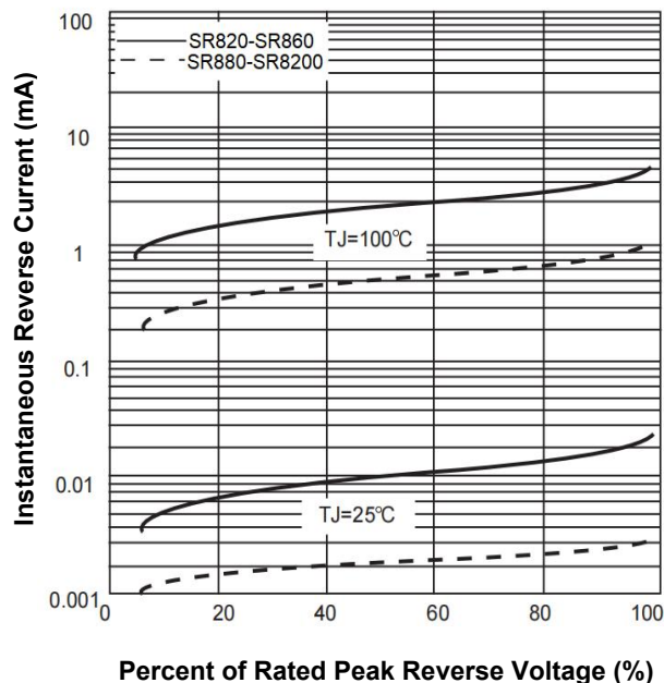
FIG. 4- TYPICAL REVERSE LEAKAGE
