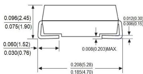
Package Outline Dimensions in Inches (Millimeters)
